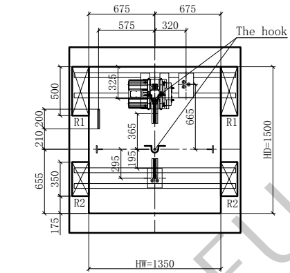
Overhead plan
