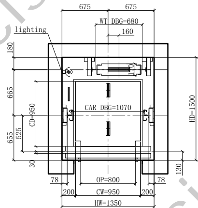
Hoistway plan
