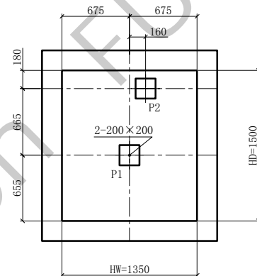
Pit plan
