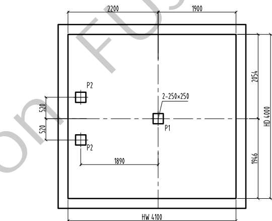
Pit plan/1: 60
