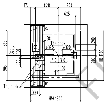
Overhead plan/1:60
