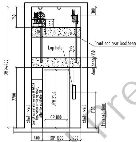
E/reserved hole/1: 60
