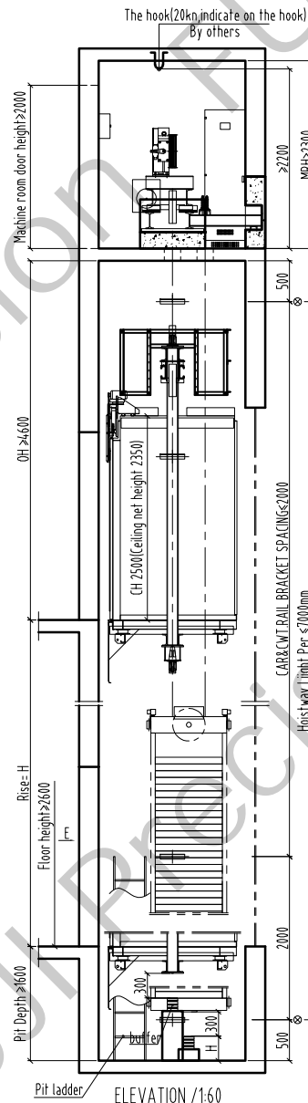
ELEVATION /1:60
