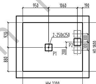
Pit plan/1: 60
