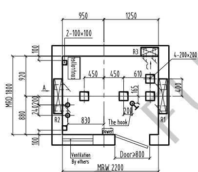
Machine room plan/1:60
