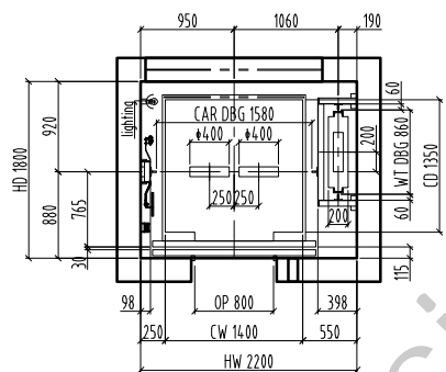
Hoistway plan/1:60
